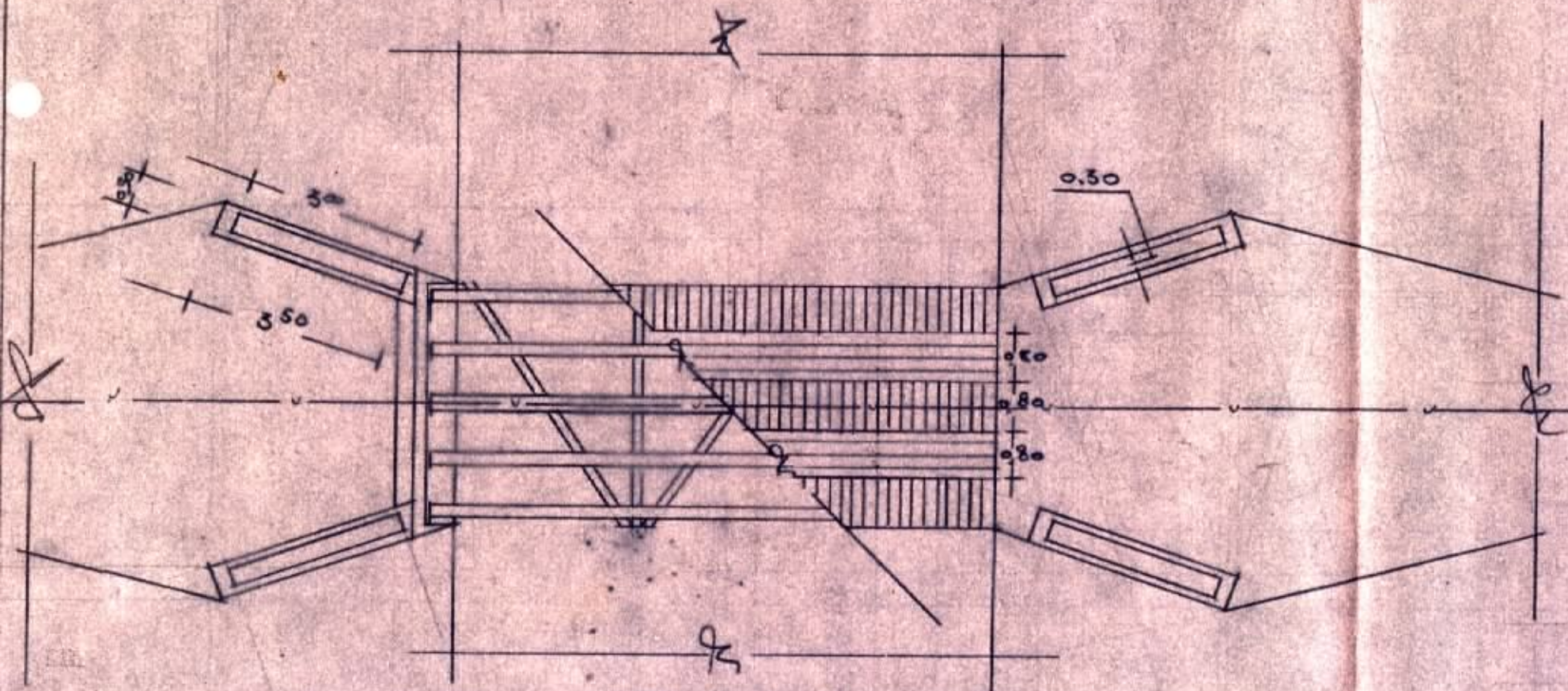
DENAH.
